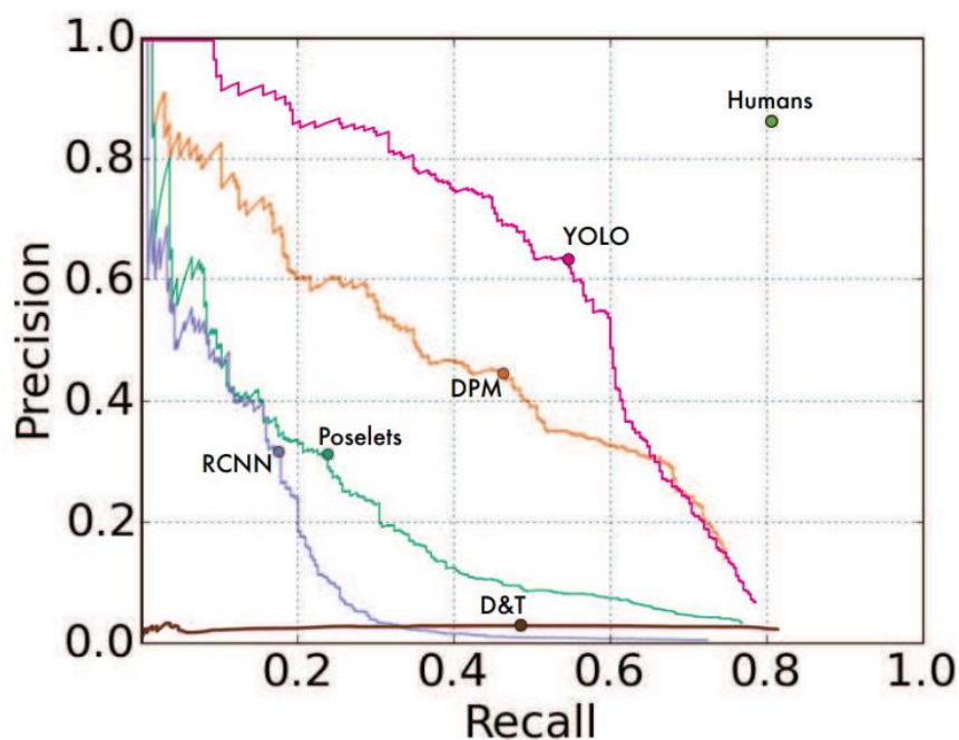
Figure A1.4.1 Picasso Dataset precision-recall curves
