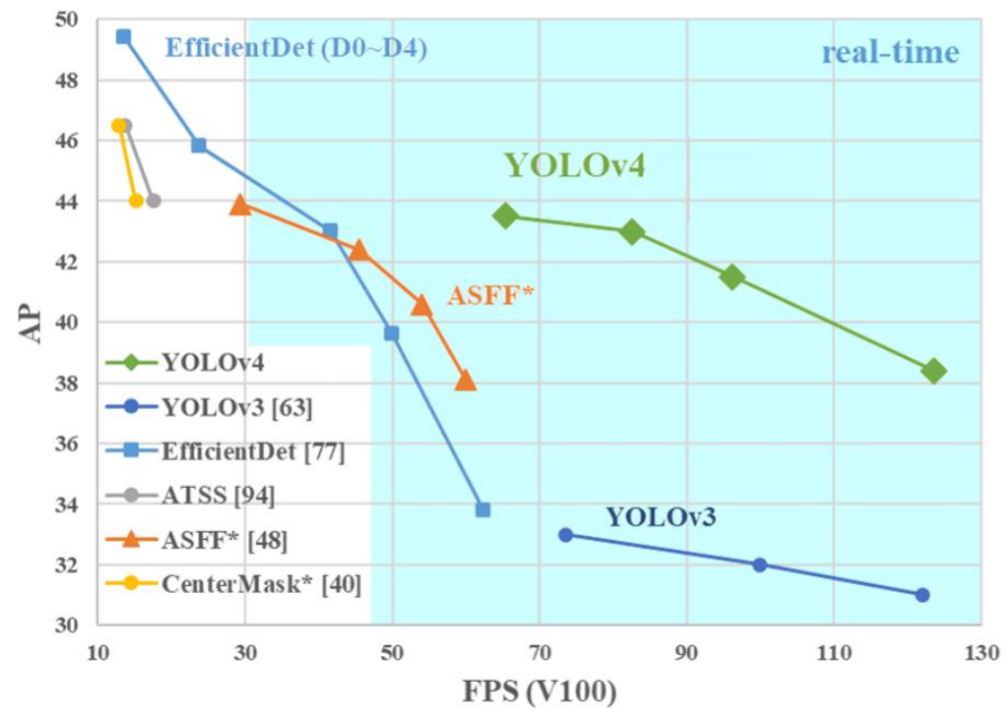
Figure A1.4.2 Comparison of YOLO models
