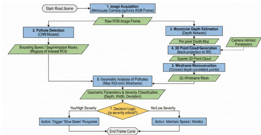
Figure 3.2.3 Monocular Vision Algorithm Architecture
